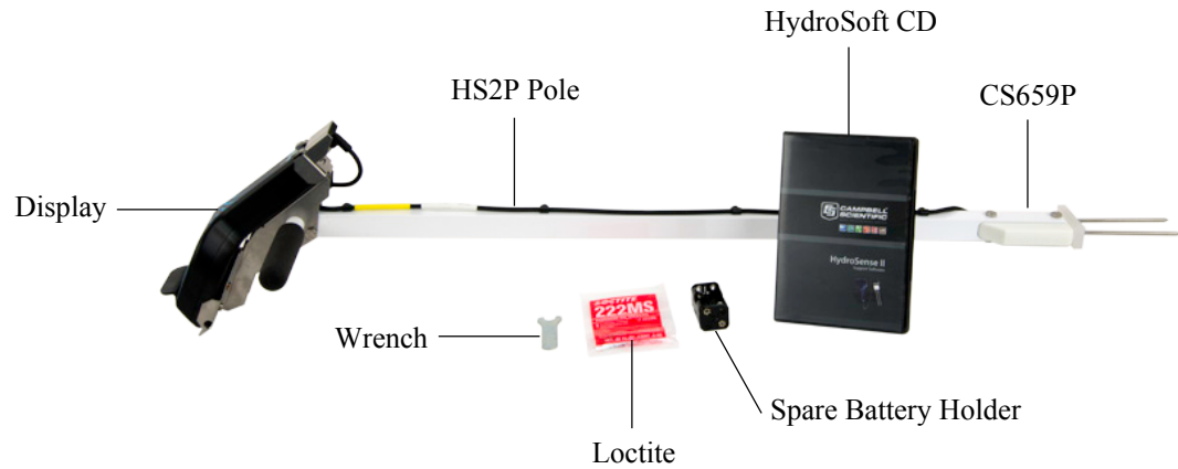
FIGURE 4-3. HS2P Parts
