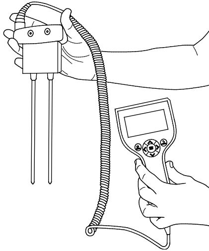
FIGURE 1-1. HS2 HydroSense II System
